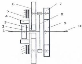
1. Engine shaft. 2. Generator rotor. 3. Central gear of the differential. 4. Generator "stator" winding. 5. Link. 6,7. Satellites. 8. Carrier. 9. Second central gear. 10. Driven shaft
