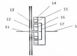
11. Input shaft. 12. Disc of input of the clutch. 13. Mating disc of the coupling. 14. Crown of the planetary gear. 15. Satellites. 16. Central gear. 17. Carrier. 18. Driven shaft.
