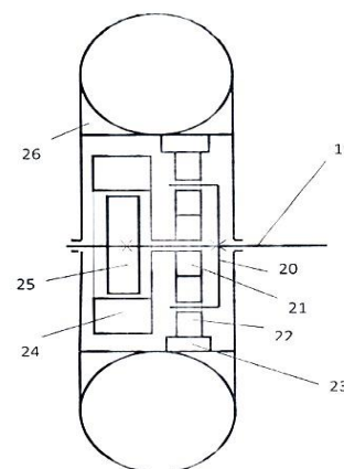
19. Motor shaft. 20. Carrier. 21. Central wheel. 22 Satellites. 23. Crown. 24. Inductor. 25. Armature of the electromagnetic clutch. 26. Wheel.
