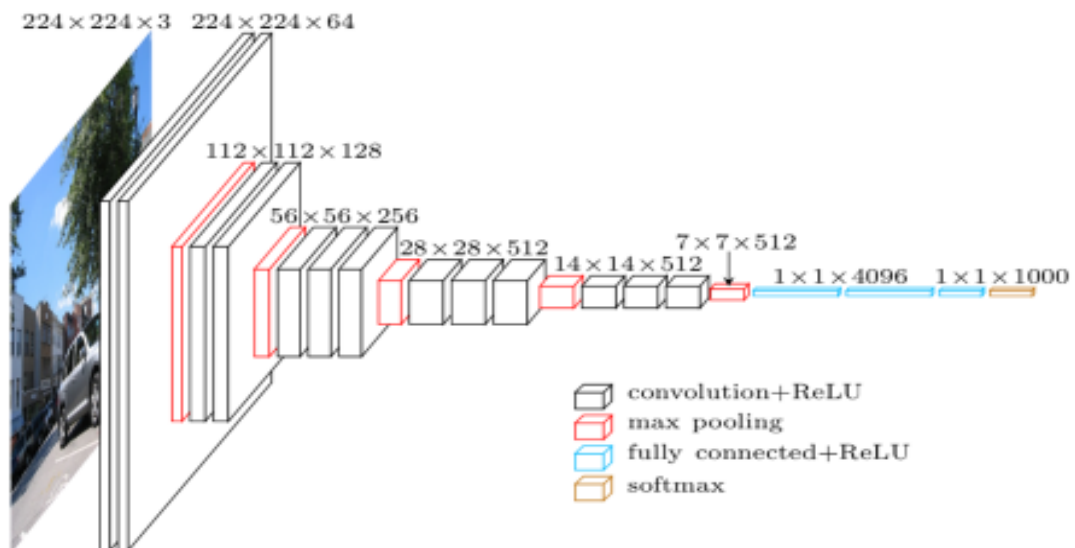
Fig. 3: VGG-16 Architecture [75].
