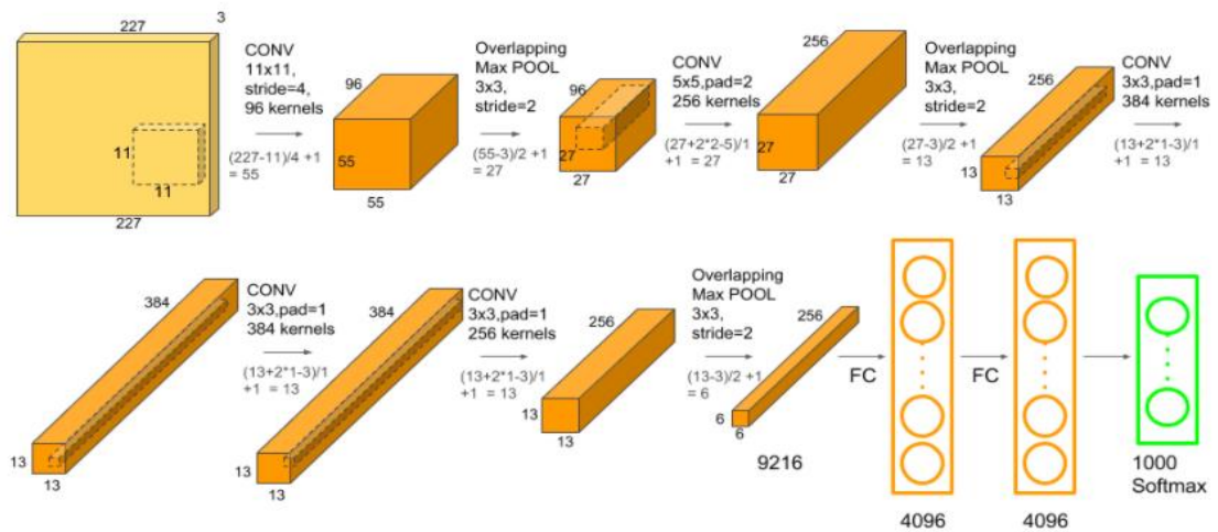
Fig. 2: AlexNet Architecture [57]
