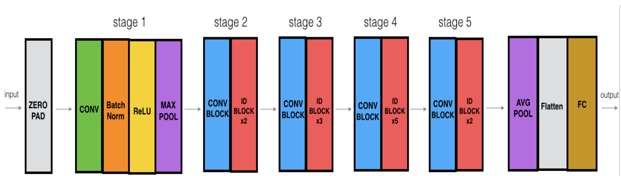
Fig. 6: ResNet50 model [66]
