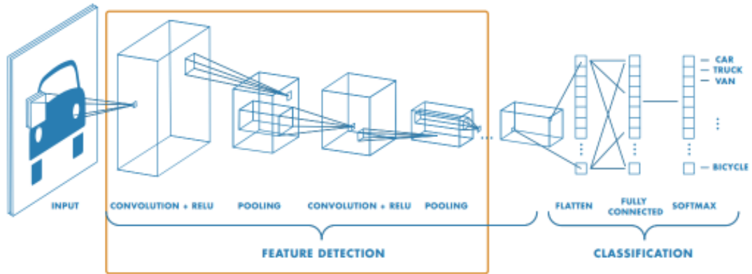
Fig. 1: CNN Architecture [100]
