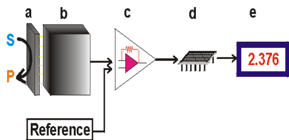
Fig. 6. Schematic diagram showing the main components of a biosensor. The biocatalyst (a) converts the substrate to a product. This reaction is determined by the transducer (b) which converts it to an electrical signal. The output from the transducer is amplified (c), processed (d) and displayed (e) (Chaplin, 2004).
