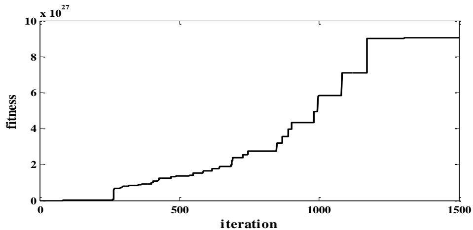
Fig 6. Fitness variation versus GA number of iteration in case2
