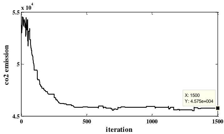
Fig 4. CO2 emission versus GA number of iterations in case 1
