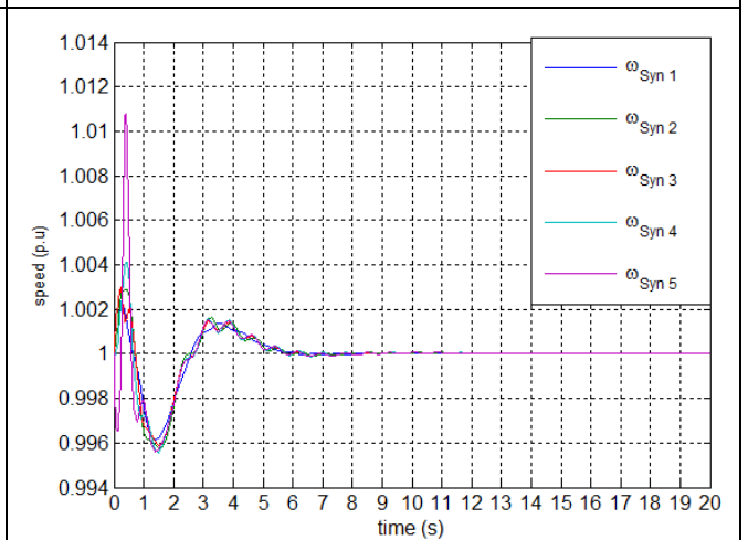
Fig. 8. The speed (omega) of all generators –fault at buss 11 –no wind energy in the system-
